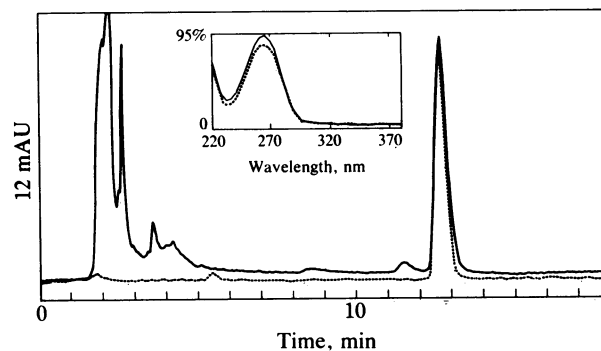
FIG. 1. Identification of the product derived from HI reduction of rat thymine glycol fraction 2 as thymine. A pool of rat thymine glycol fraction 2 samples was reduced with HI, and the peak corresponding to presumptive thymine was purified from the reaction mixture. The purified thymine (fraction 3) was then chromatographed on a 5- \mu m C18 column at 35°C and a H 2 O flow rate of 1 ml/min, using a Hewlett-Packard 1040a photodiode array detector. The chromatogram demonstrates comigration of 1 nmol of thymine standard (broken line) with the product obtained by HI reduction of thymine glycol fraction 2 (solid line). The detector was scanning at 260 nm with a bandpass of 20 nm. (Inset) Spectra acquired at the apex of the comigrating peaks in the chromatogram: broken line, thymine standard; solid line, HI reaction product. \lambda_{\max} for each peak was 265 nm.
