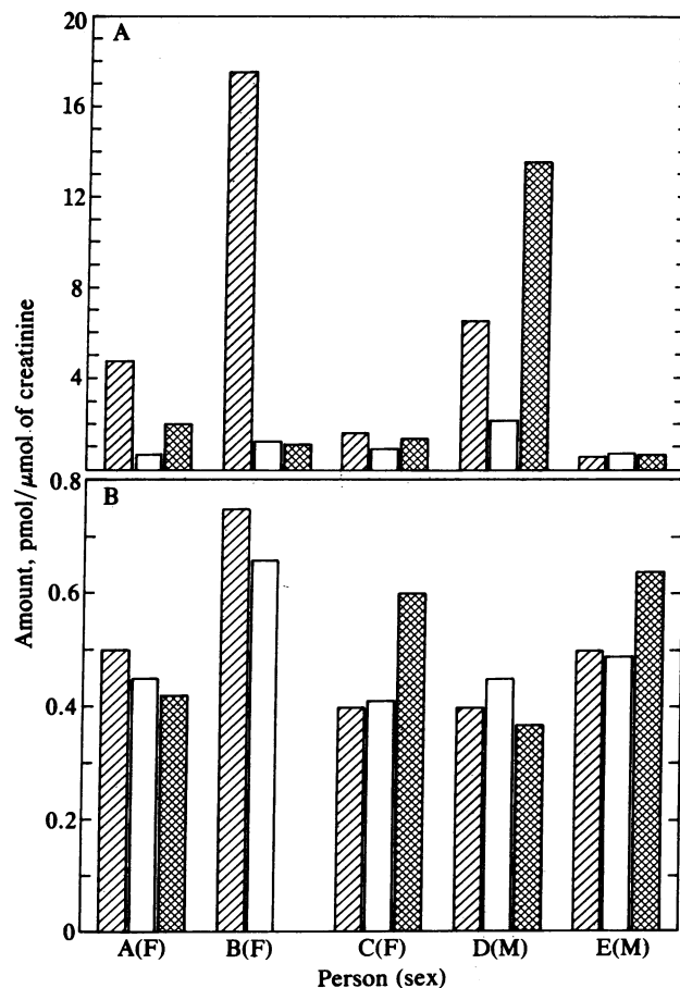
FIG. 2. Variation in human thymine glycol (A) and thymidine glycol (B). Bars: ▨, day 1, morning; □, day 2, morning; ▩, day 2, 24-hr sample. Each day 1, morning urine level, is the mean of four separate determinations, with a SEM per sample of less than 15%. Day 2 levels are results of single determinations. The 24-hr sample of thymidine glycol, person B, was lost.
