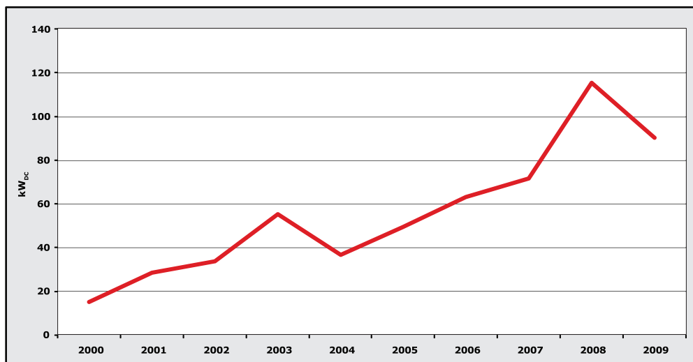
Fig. 4: Average Capacity of U.S. Grid-Connected Non-Residential PV Installations (2000-2009)
