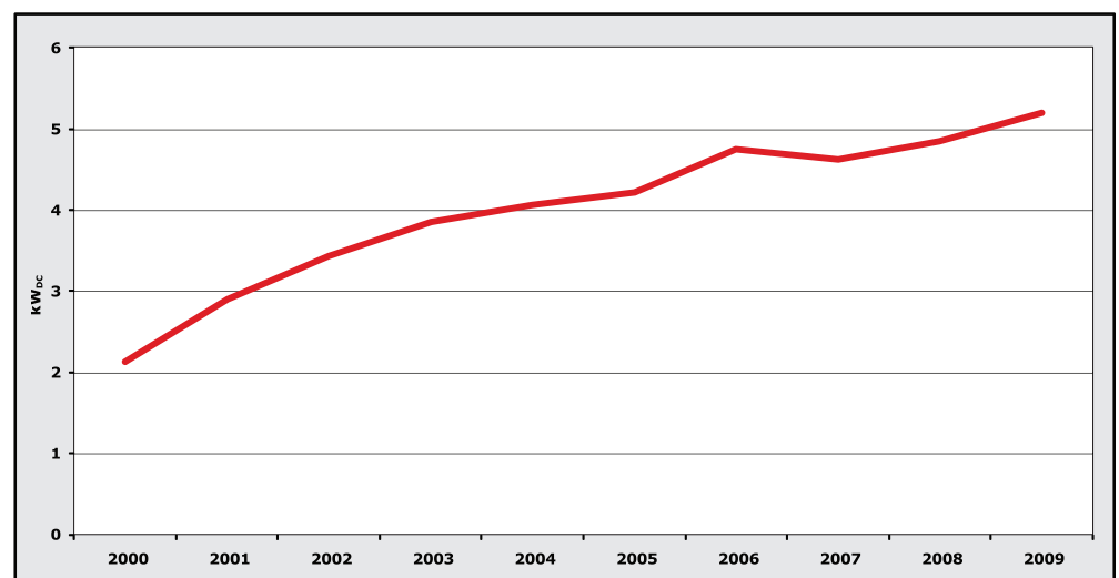
Fig. 3: Average Capacity of U.S. Grid-Connected Residential PV Installations (2000-2009)
