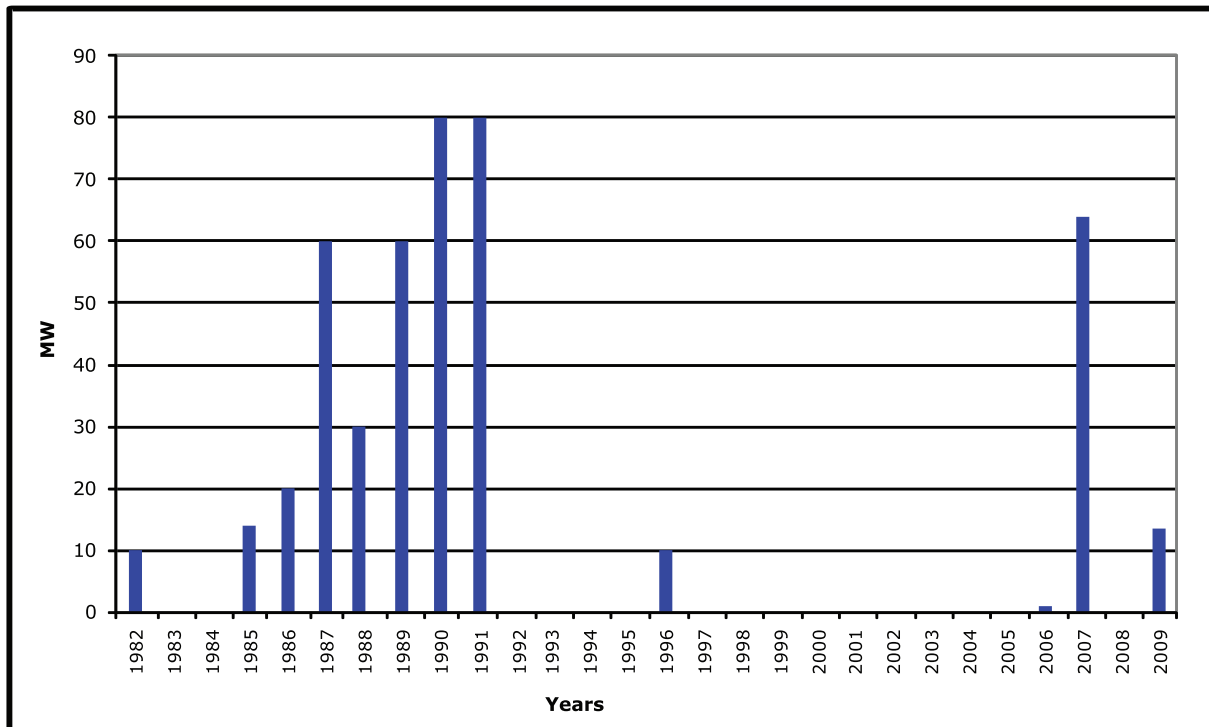
Fig. 6: Annual Installed U.S. CSP Capacity (1982-2009)
