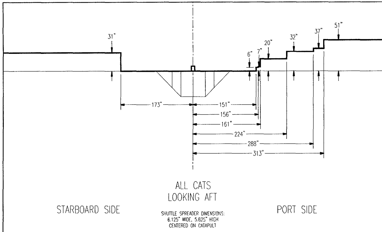
Figure 4: Composite Catapult Clearance Envelope, CVN-68 Class
