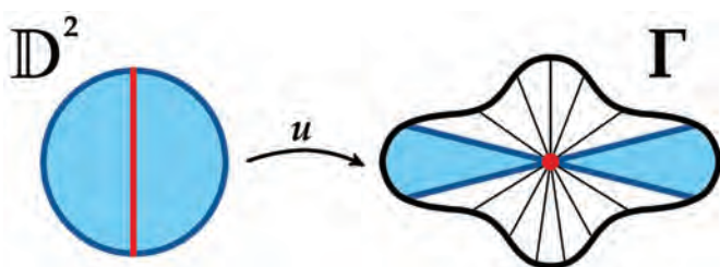
Figure 44. The singular set S(u) (depicted in red on the left) of the energy-minimizing map u from a disk, \mathbb{D}^2 , into a cone, Cone(\Gamma) , over a curve, \Gamma , of length greater than 2\pi , with prescribed boundary (in dark blue), has Hausdorff dimension at least 1.
