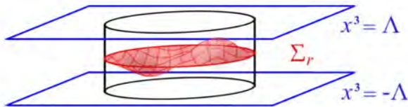
Figure 10. In their proof of the positive mass theorem, Schoen and Yau find a least area surface, \Sigma_r , with boundary, \partial\Sigma_r , lying in a cylinder of radius r , before taking r \rightarrow \infty to create a complete stable minimal surface.
