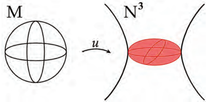
Figure 17. The standard map from M = \mathbb{S}^2 into the horizon at the neck of Schwarzschild space N^3 is a harmonic map as well as minimal.
