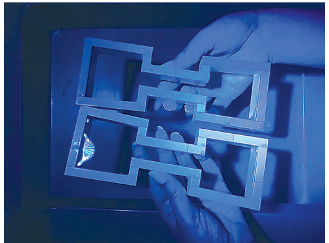
Figure 29. Connected minimal surfaces with these nonconvex boundaries are depicted in Figures 30–31.
