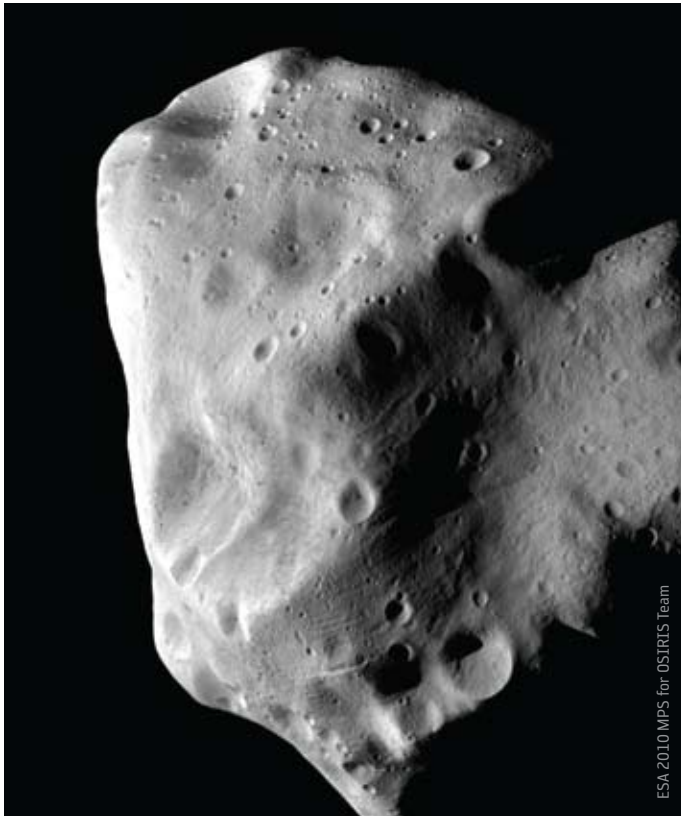
Asteroid Lutetia, as seen by ESA's Rosetta in 2010
