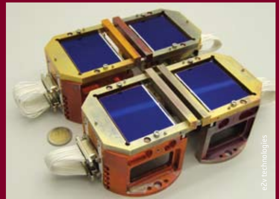
Four of the 106 CCDs that are part of Gaia's large focal plane
