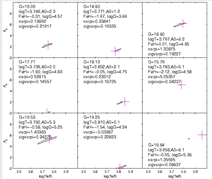
Figure 2. GSP-Phot output for T_{eff} - A_0 , which are degenerate. T_{eff} is star effective temperature and A_0 is the first parameter of the extinction curve. The contour bounds the 90% likelihood interval and the cross marks the true values of T_{eff} and A_0 .
