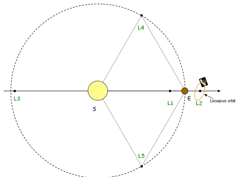
Qualitative positions of the Lagrangian points for the Sun-Earth system (Figure not to scale).
