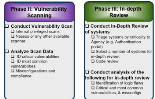
Figure 4. Vulnerability and in-depth review phases
