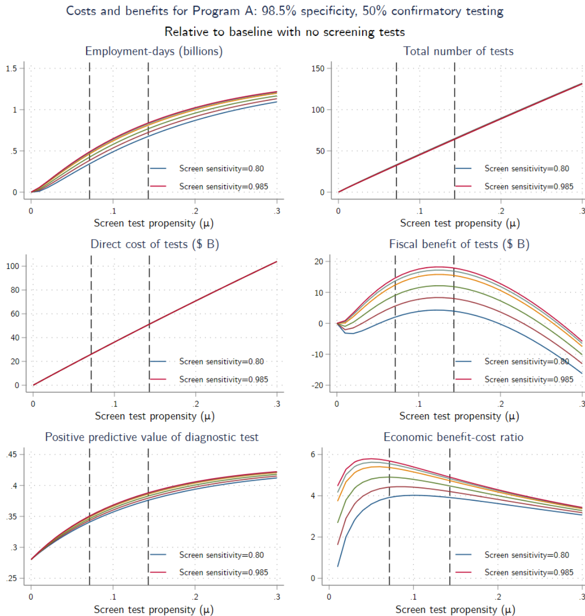
Figure 4. Costs and benefits for program A (50% confirmatory PCR testing)
