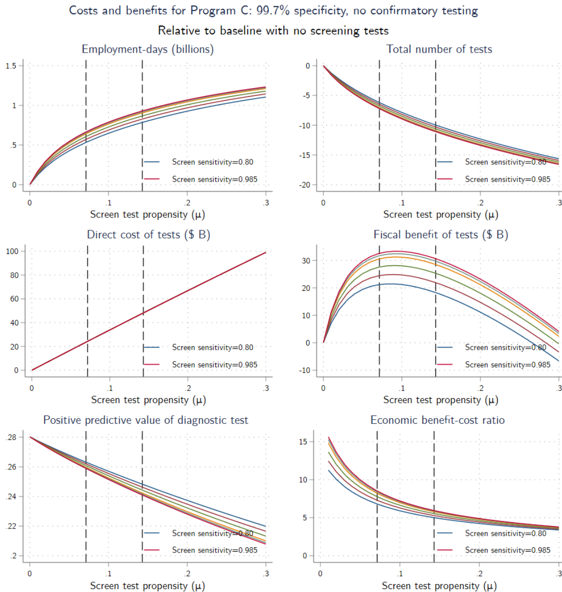
Figure 8. Costs and benefits for program C (no confirmatory PCR testing)
