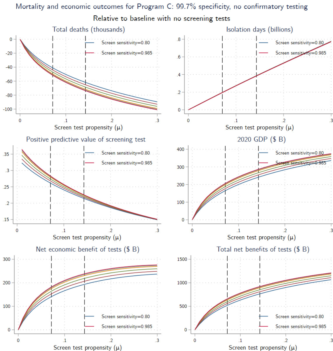
Figure 7. Mortality and economic outcomes for program C (no confirmatory PCR testing)
