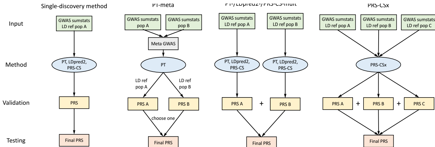
Figure 1: Overview of polygenic prediction methods. The predictive performances of three representative single-discovery methods: (i) LD-informed pruning and p -value thresholding (PT); (ii) LDpred2; (iii) PRS-CS; and five multi-discovery methods: (i) PT-meta; (ii) PT-mult; (iii) LDpred2-mult; (iv) PRS-CS-mult; (v) PRS-CSx are compared in this study. The discovery samples (to generate GWAS summary statistics), validation samples (to turn hyper-parameters in PRS construction methods) and testing samples (to assess prediction accuracy) are non-overlapping. LD ref: LD reference panel; pop A/B/C: Population A/B/C.
