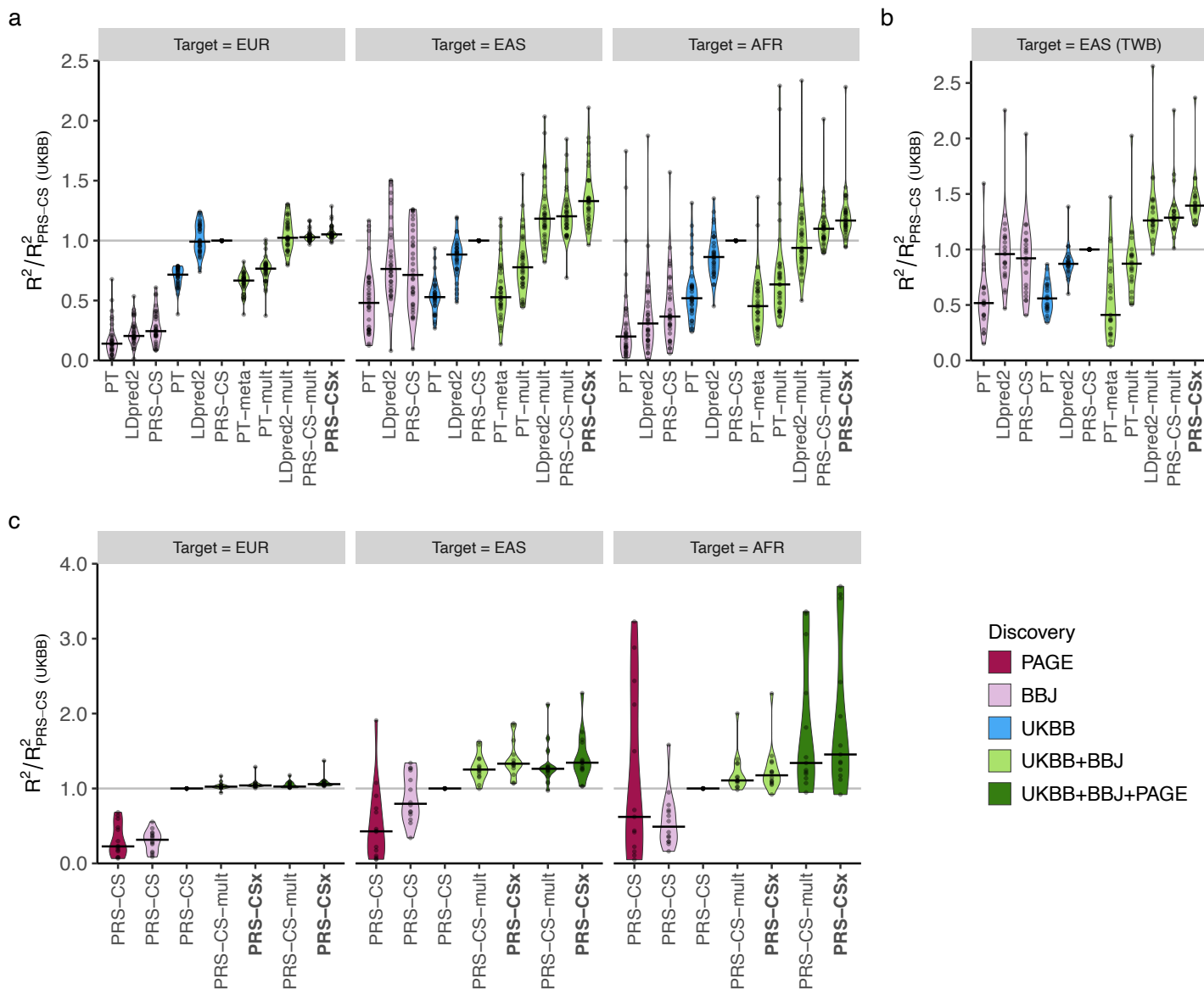
Figure 3: Prediction accuracy of quantitative traits using GWAS summary statistics from UKBB, BBJ and PAGE. (a) Relative prediction accuracy of single-discovery and multi-discovery polygenic construction methods using GWAS summary statistics from UKBB and BBJ, with respect to PRS-CS trained on the UKBB GWAS, across 33 traits in different UKBB target populations (EUR, EAS and AFR). Each data point shows the relative prediction R^2 of a trait, averaged across 100 random splits of the target samples into validation and testing datasets. (b) Relative prediction accuracy of different polygenic prediction methods using discovery GWAS from UKBB and BBJ, with respect to PRS-CS trained on the UKBB GWAS, across 21 traits in the Taiwan Biobank (TWB). Each data point shows the relative prediction R^2 of a trait. (c) Relative prediction accuracy of PRS-CS, PRS-CS-mult and PRS-CSx using discovery GWAS from UKBB, BBJ and PAGE, with respect to PRS-CS trained on the UKBB GWAS, across 14 traits in different UKBB target populations (EUR, EAS and AFR). Each data point shows the relative prediction R^2 of a trait, averaged across 100 random splits of the target samples into validation and testing datasets. MCHC was removed from the AFR panel due to the near-zero R^2 of PRS-CS (UKBB) and thus inflated relative prediction R^2 for other methods. In all panels, the crossbar indicates the median of relative R^2 across traits examined.
