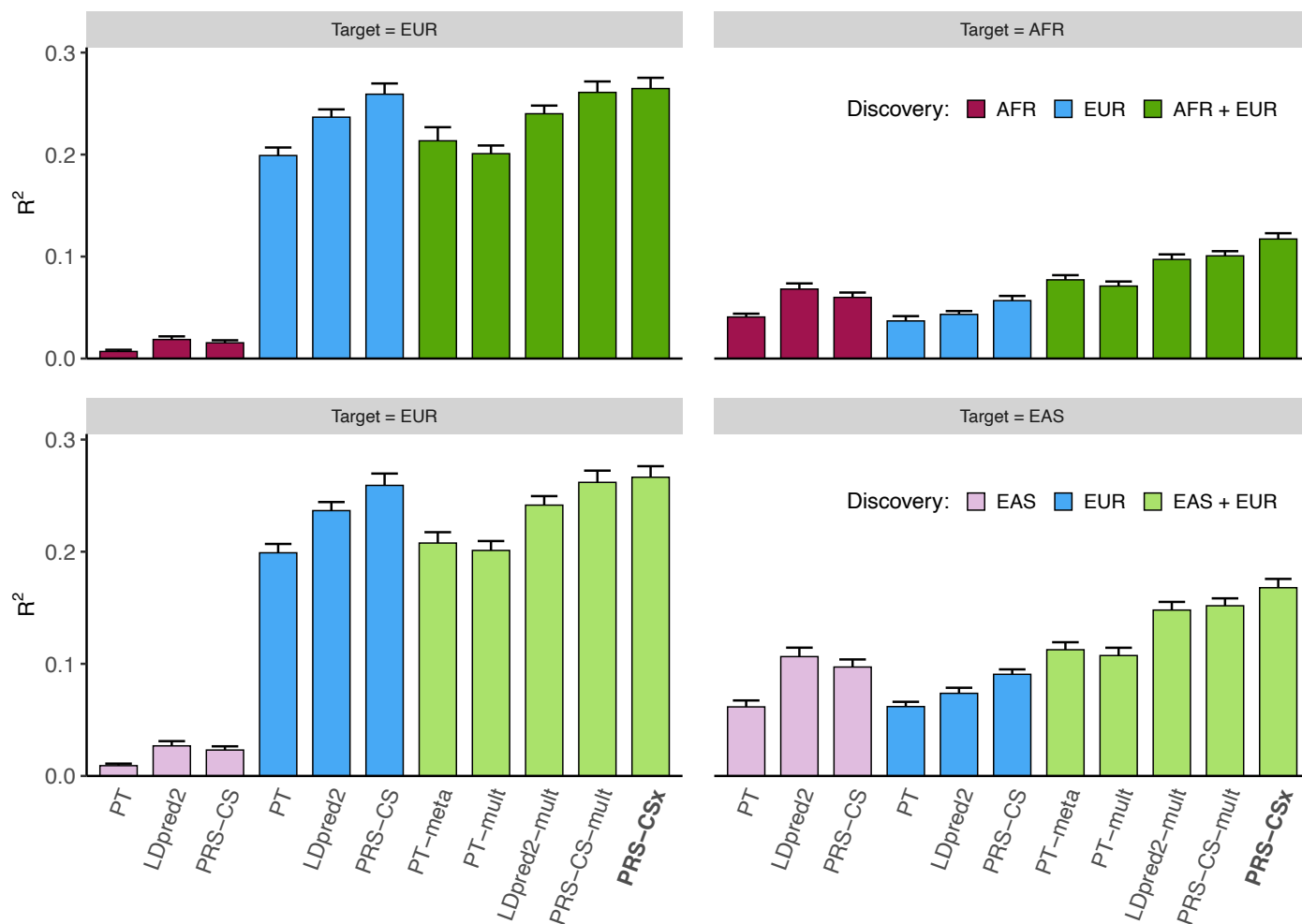
Figure 2: Prediction accuracy of single-discovery and multi-discovery polygenic prediction methods in simulations. 1% HapMap3 variants were randomly sampled as causal variants, which in aggregation explained 50% of phenotypic variation in each population. Causal variants were shared across populations with a cross-population genetic correlation of 0.7. 100K simulated EUR samples and 20K non-EUR (EAS or AFR) samples were used as the discovery dataset. Prediction accuracy was measured by the squared correlation ( R^2 ) between the simulated and predicted phenotypes in an independent testing dataset, averaged across 20 simulation replicates. Error bar indicates the standard deviation of R^2 across simulation replicates.
