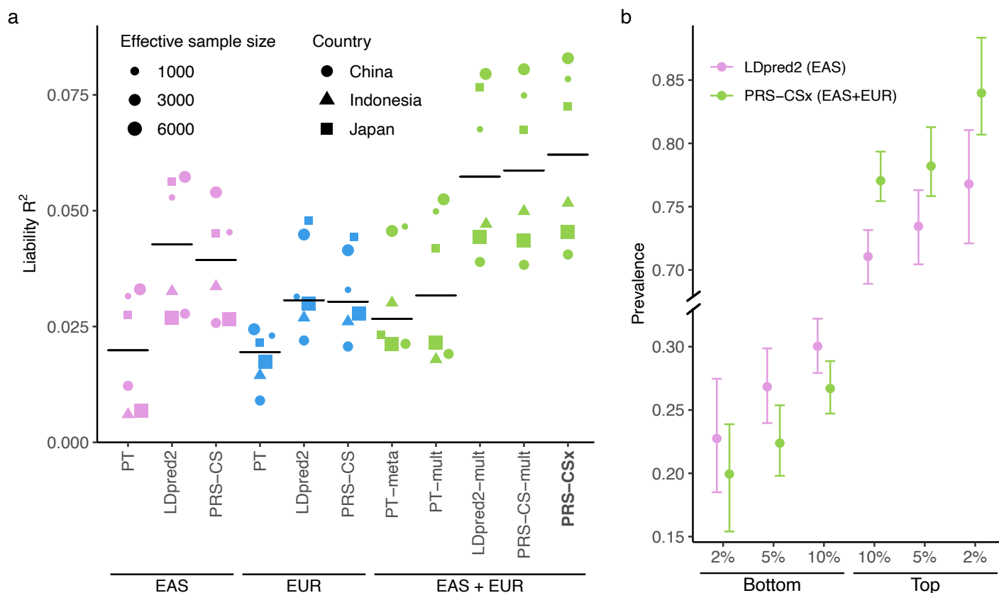
Figure 4: Prediction accuracy of schizophrenia risk in EAS cohorts. (a) Prediction accuracy, measured as R^2 on the liability scale, of single-discovery (trained on EAS or EUR GWAS) and multi-discovery polygenic prediction methods (trained on both EAS and EUR GWAS: EAS+EUR) across 6 EAS schizophrenia cohorts. Each dot represents one testing cohort, with the size of the dot proportional to the effective sample size, calculated as 4(1/N_{case}+1/N_{control}) , and the shape of the dot representing the country where the sample was collected. Crossbar indicates the median R^2 on the liability scale. (b) Case prevalence of the bottom 2%, 5%, 10% and top 2%, 5%, 10% of the PRS distribution, constructed by LDpred2 trained on EAS GWAS (the best-performing single-discovery method) and PRS-CSx (the best-performing multi-discovery method), across 6 EAS schizophrenia cohorts. Error bar indicates 95% confidence intervals.
