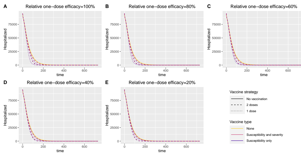
Figure S3: Predicted hospitalizations if NPIs are sustained at their current level for the duration of the simulation (2 years)
