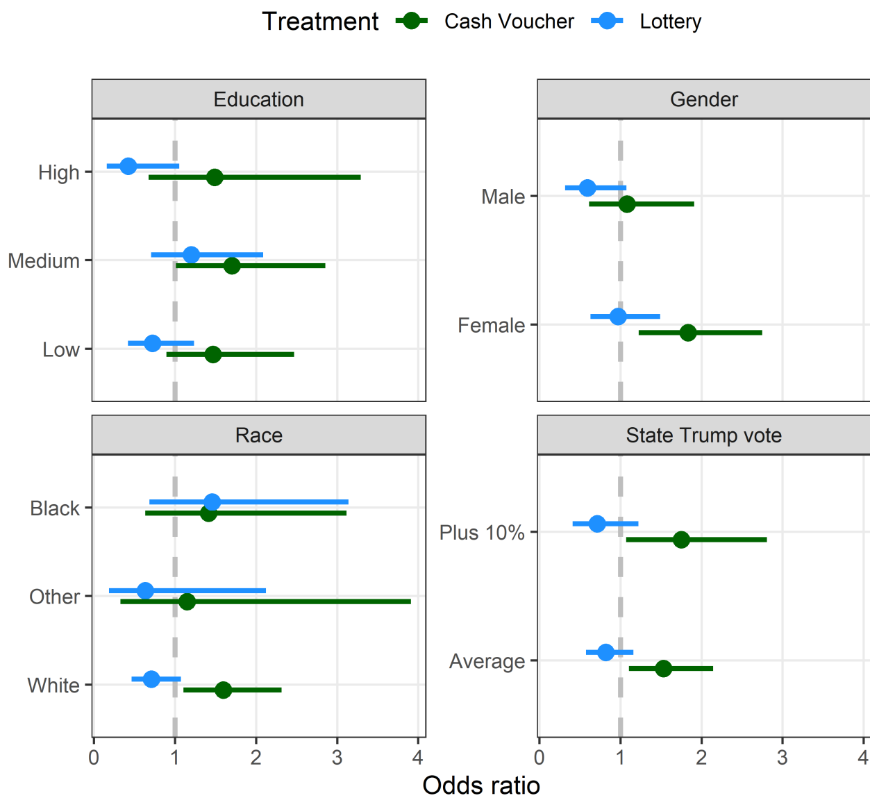
Figure 3: Estimated odds ratios and 95% credible intervals of the treatment effect interacted with with gender, race, education and state Trump vote from the Bayesian Logistic Regression Model
