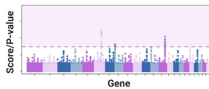
Gene prioritization
