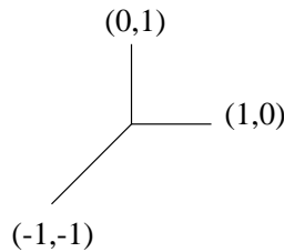
FIGURE 1. The fan for \mathbb{C}\mathbb{P}^2
