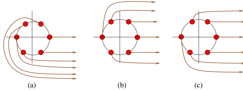
FIGURE 19. Three exceptional collections.
