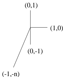
FIGURE 2. The fan for F_n
