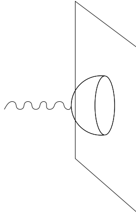
FIGURE 3. Disc diagram for graviton emission from D-brane
