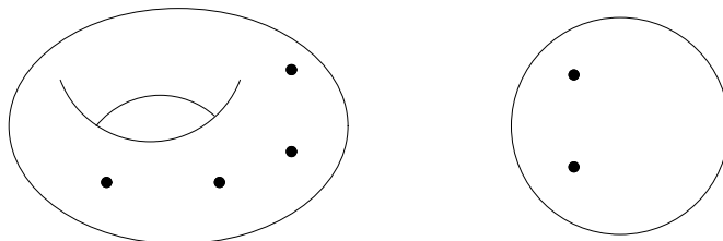
FIGURE 3. The normalization of the curve in Fig. 2, with node-branches marked
