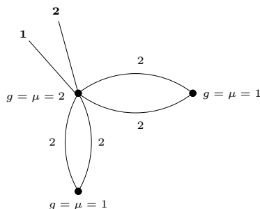
FIGURE 1. An example of a marked graph \Gamma corresponding to a component of \overline{\mathcal{M}}_{6,2}(\mathbb{P}^2, 8) ( \# \text{Aut } \Gamma = 8 , \# \mathbb{A}_\Gamma = 2^4 \cdot 8 )
