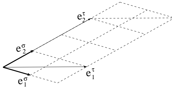
FIGURE 1. Lattice configurations that allow for a degree 6 map.
