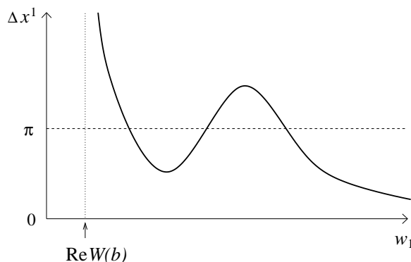
FIGURE 11. A graph of \Delta x^1 as a function of w_1 = \operatorname{Re} A = \operatorname{Re} B . Corresponding to the situation in Fig. 10, the left end is set at w_1 = \operatorname{Re} W(b) .
