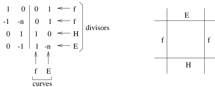
FIGURE 4. Divisors and intersections on F_n
