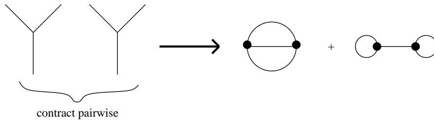
FIGURE 1. There is one vertex for each X^3 and the three edges emanating from the vertex are in one-to-one correspondence with the three X 's
