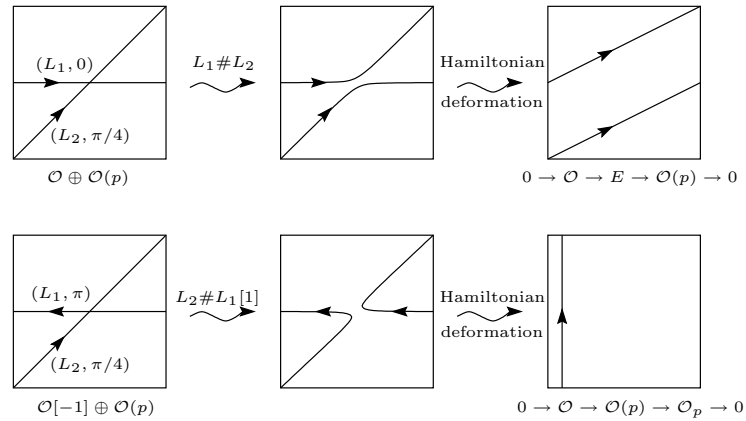
FIGURE 3. L_1 \# L_2 , L_2 \# L_1[1] , equivalent sLags, and mirror sheaves
