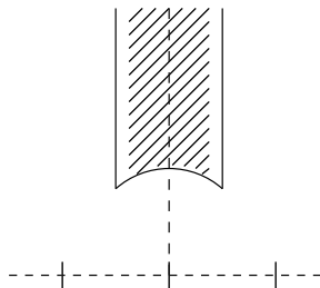
FIGURE 1. The moduli space of an elliptic curve.
