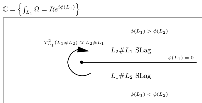
FIGURE 1. \left(\int_{L_1} \Omega\right) -space in a K3 , with polar coordinates (R, \phi(L_1))
