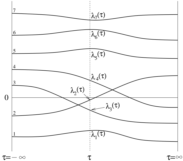
FIGURE 8. The Spectral Flow: An example for the case \dim M = 7 . The Morse index at x_i is \mu_i = 2 whereas that at x_j is \mu_j = 3 . One of the eigenvalues ( \lambda_2(\tau) ) goes from negative to positive but two of them ( \lambda_3(\tau) and \lambda_4(\tau) ) go from positive to negative
