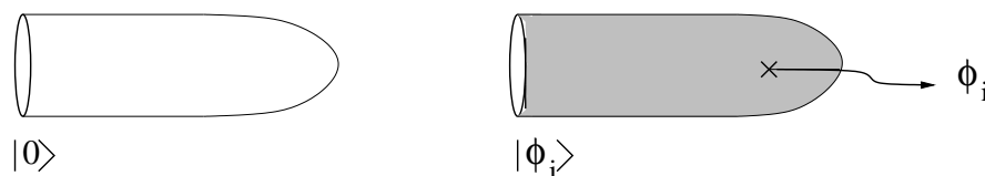
FIGURE 2. The topological path-integral on a hemisphere attached to a semi-infinite tube results in a ground state at the boundary. For each chiral operator \phi_i we obtain a corresponding ground state |i\rangle given by the path-integral
