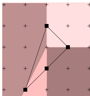
FIGURE 2. The fan for F_2
