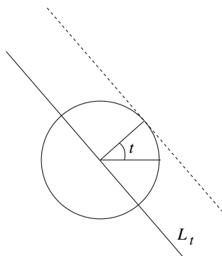
FIGURE 5. The Lagrangian subspace L_t
