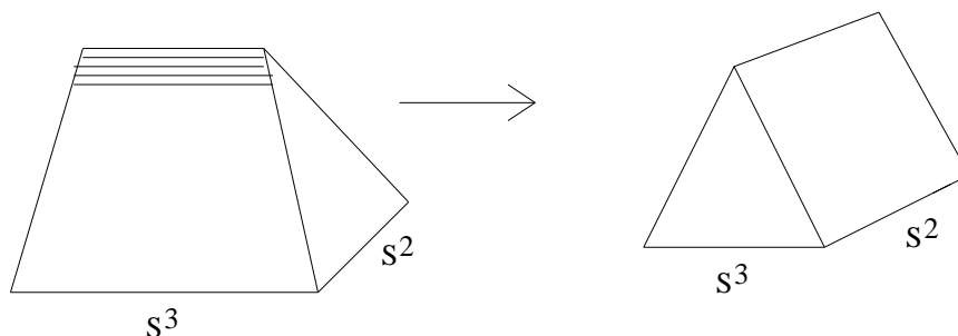
FIGURE 4. Conifold singularity resolved by blowing up S^2
