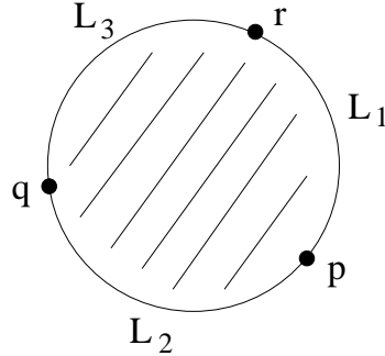
FIGURE 3. Holomorphic maps contributing to m_2((p, a), (q, b)) , where (p, a) \in \text{Hom}(\mathcal{U}_1, \mathcal{U}_2) — i.e., p \in L_1 \cap L_2 and a \in \text{Hom}(E_1, E_2)|_p , — and (q, b) \in \text{Hom}(\mathcal{U}_2, \mathcal{U}_3) . The composition is given by a sum over maps \phi satisfying the boundary conditions pictured, and is m_2((p, a), (q, b)) = \sum_{r \in L_1 \cap L_3} \pm e^{2\pi i \int \phi^* \omega} \cdot P e^{2\pi i \oint \phi^* \beta} , where \beta is the connection on the boundary formed by the connections on L_1, L_2, L_3 , linked by p and q , as described in the text.
